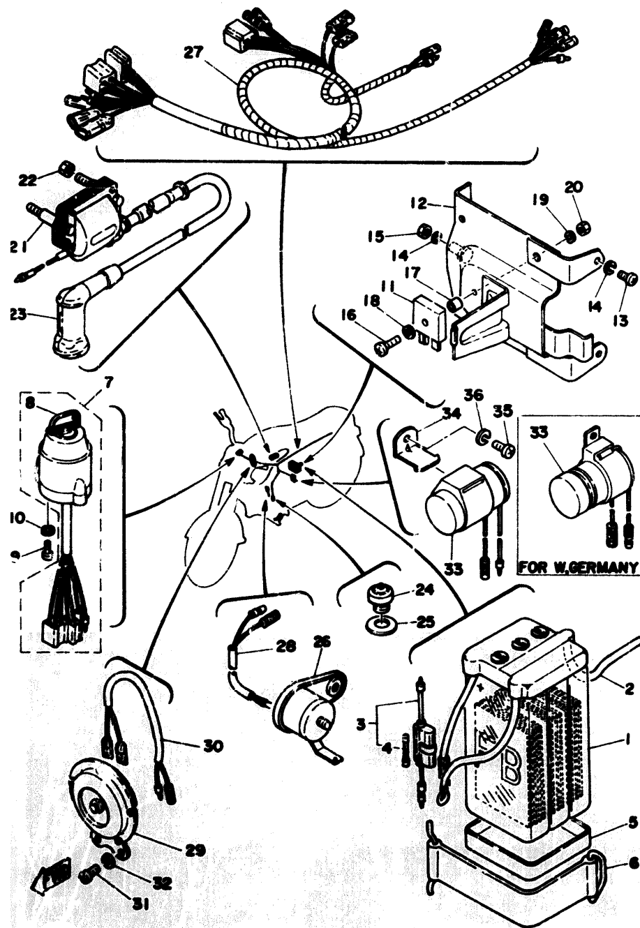
Fig. 39 ELECTRICAL
