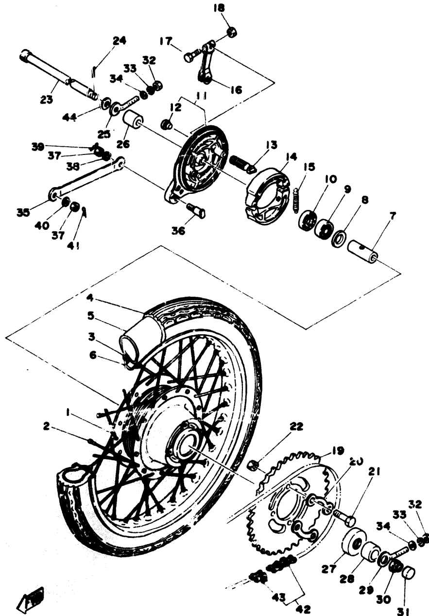
Fig. 31 REAR WHEEL
