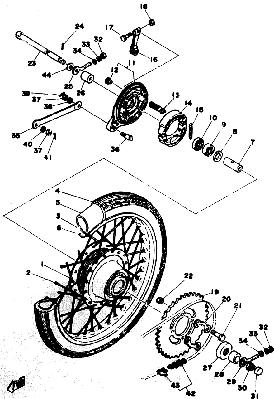
Fig. 31 REAR WHEEL
