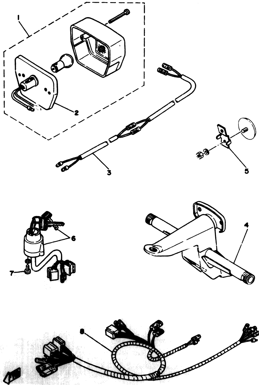
Fig. 4 TAIL LAMP - ELECTRICAL
