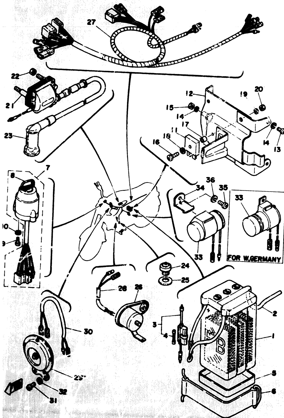
Fig. 39 ELECTRICAL
