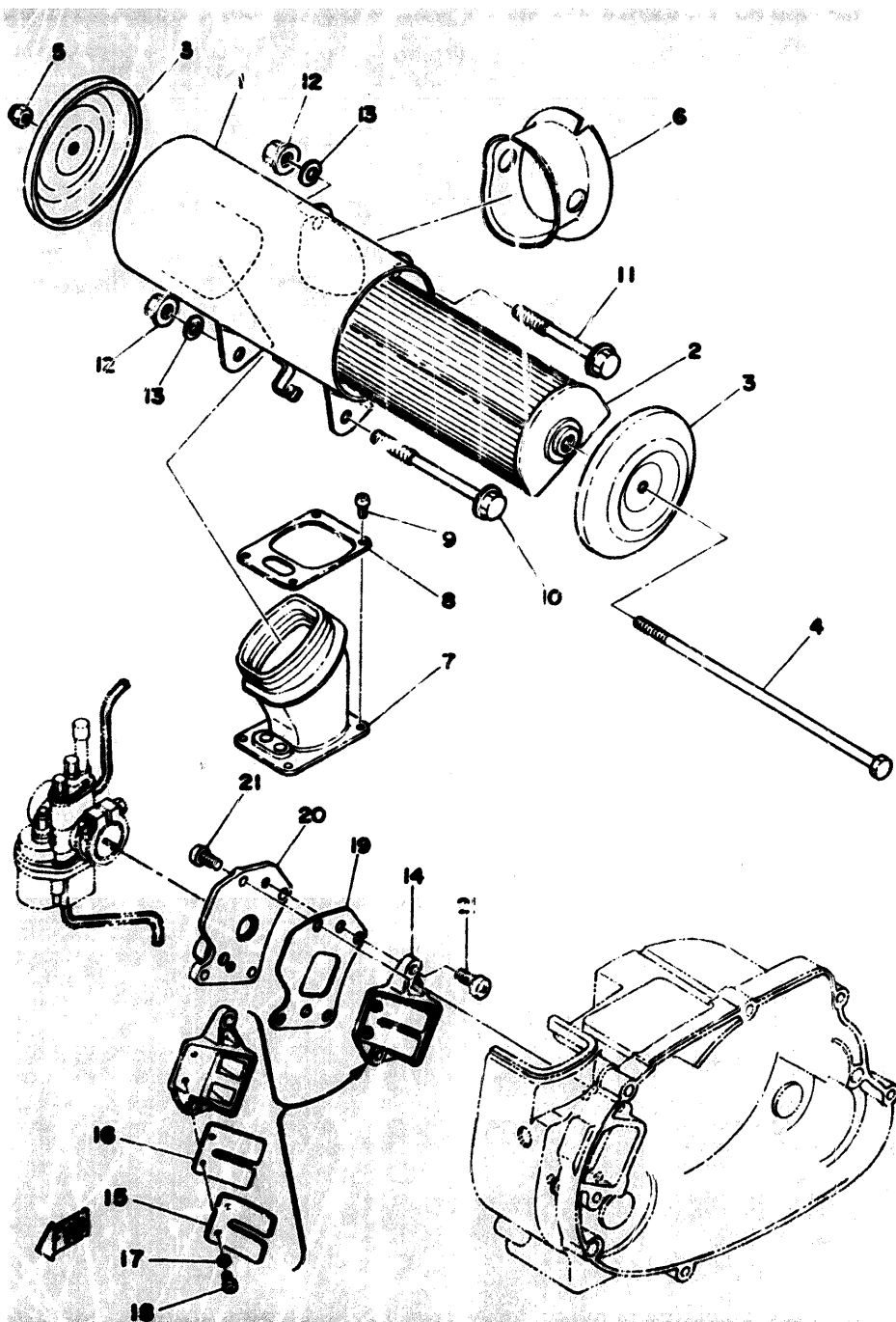
Fig. 9 INTAKE
