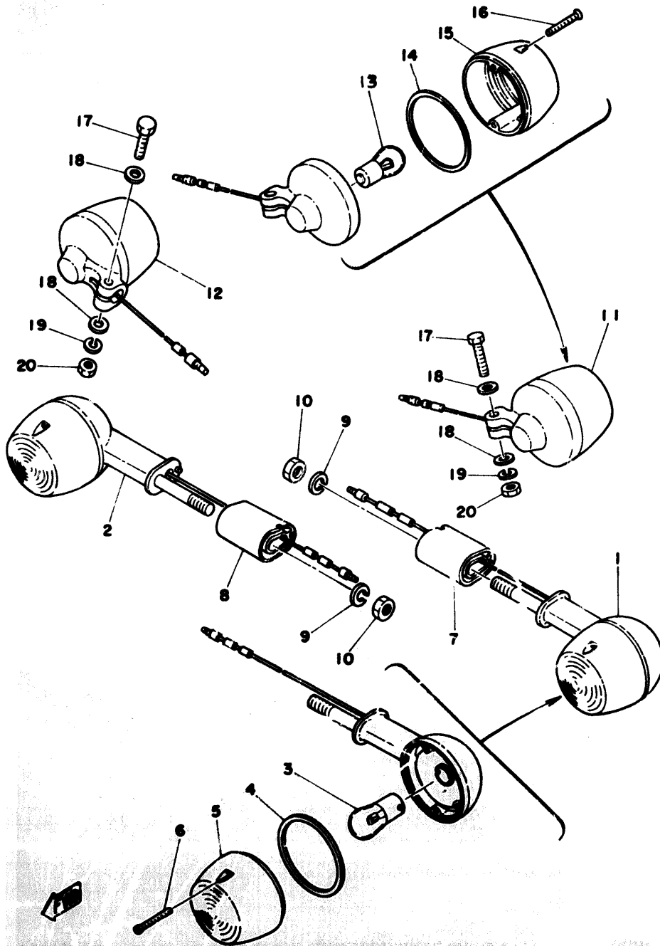
Fig. 37 FLASHER LAMP 1
