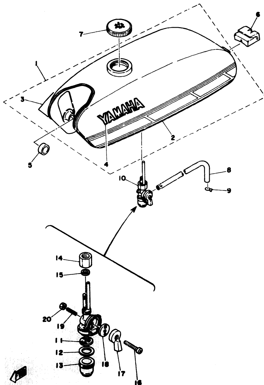
Fig. 25 FUEL TANK
