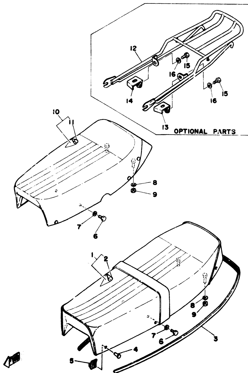
Fig. 27 SEAT
