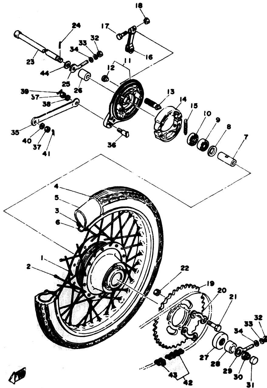
Fig. 31 REAR WHEEL
